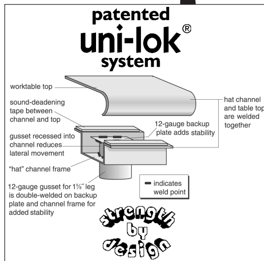
worktable with flat top and undershef
